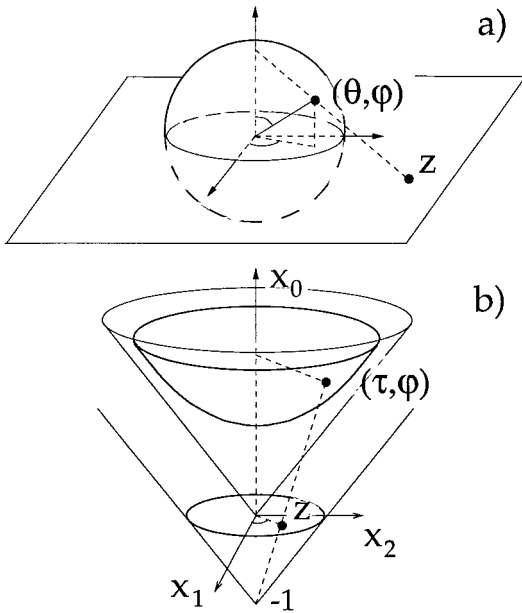
Fig. 1. (a) The sphere and, (b) the pseudosphere (upper sheet of the hyperboloid -x_0^2 + x_1^2 + x_2^2 = -1 ) having curvature +1 and -1 , respectively. For SU(2) , the definition of z corresponds to a stereographic projection which maps the unit sphere labeled by (\theta, \varphi) onto the equatorial complex plane labeled by z , the north pole of the sphere being the center of projection. In the case of SU(1, 1) , a projection of the pseudosphere onto the unit disk in the complex z -plane located at x_0 = 0 is done through the point (x_1, x_2, x_0) = (0, 0, -1) .
