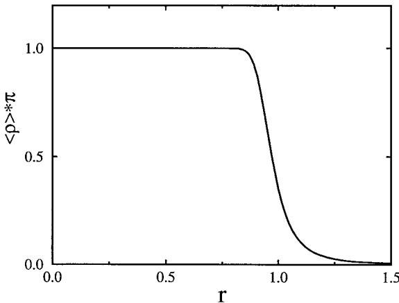
Fig. 2. The normalized density of zeros Eq. (15) for the W_1 random polynomials as a function of r = |z|/\sqrt{N\hbar} for N = 100 .
